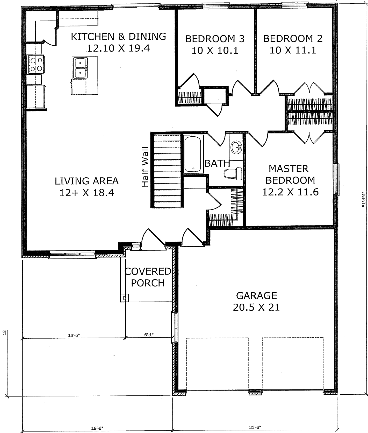
GROUND FLOOR PLAN FAIRVIEW MODEL 1260 SQ FT
